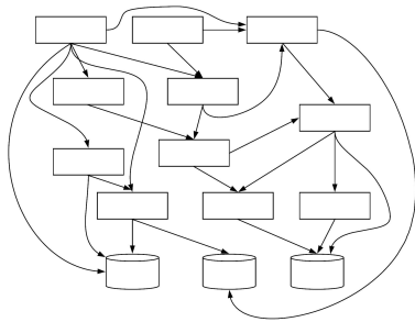
Anti-padrão big ball of mud
